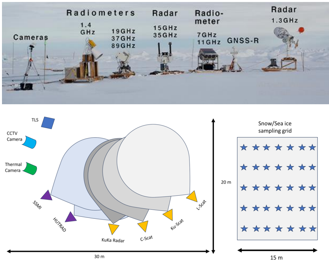
Figure 5: On-ice sampling site setup for in-situ remote sensing and snow/sea ice geophysical measurements. Top image is from MOSAiC Leg 3 Remote Sensing City (Nicolaus et al., 2022).
