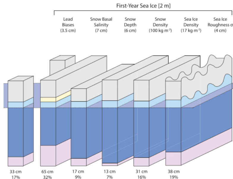
Figure 2. Schematic adapted from Landy et al., 2020 - Figure 8 illustrating the potential systematic bias in CryoSat-2-derived sea ice thickness introduced from the partial penetration of Ku-band microwaves into snow on first-year ice owing to lead detection biases, snow basal salinity, snow density, snow depth and sea ice surface roughness and sea ice density. Potential ice thickness biases are illustrated in pink for 2-metre-thick sea ice.
